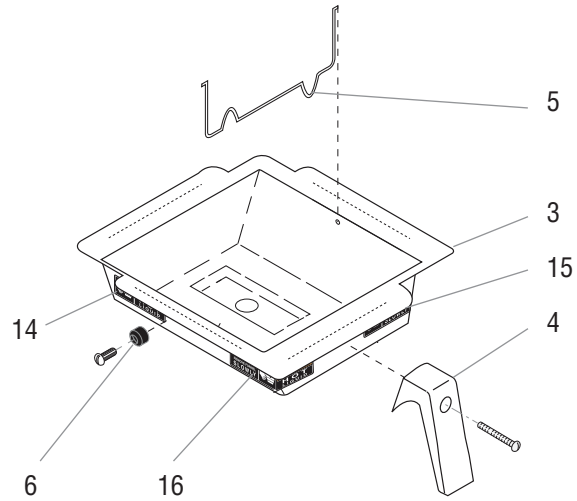
Pouch Pack Funnel
